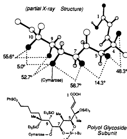
Figure 2. O–O torsion angle relationships in the C 1 –C 14 synthon.
