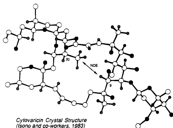
Figure 1. Transannular nuclear Overhauser effect.
