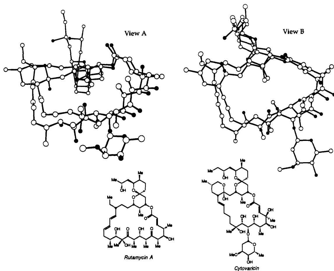
Figure 5. Superposition of rutamycin A and cytovaricin.
