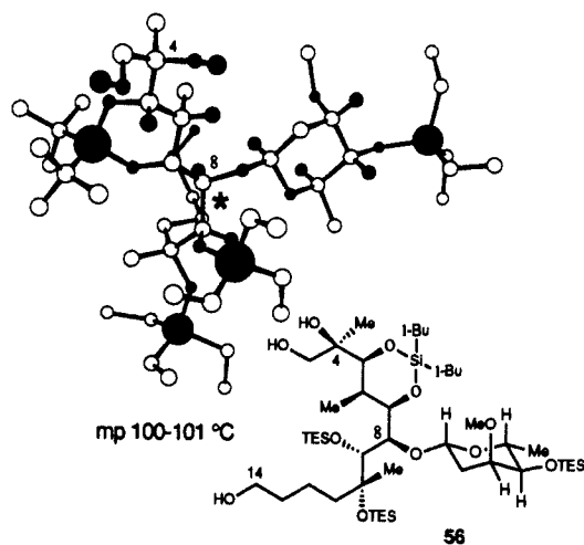
Figure 3. Crystal structure of triol 56 .
